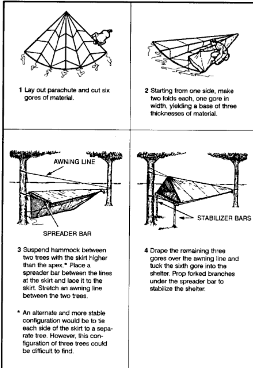
Figure 5-8. Parachute hammock.
